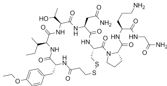
3-Mercaptopropionyl-D-Tyr(Et)-Ile-Thr-Asn-Cys-Pro-Orn-Gly-NH 2
