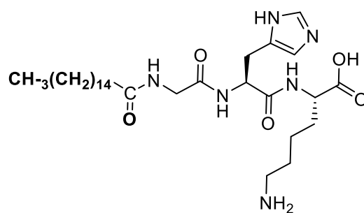
Palmitoyl-Gly-His-Lys
