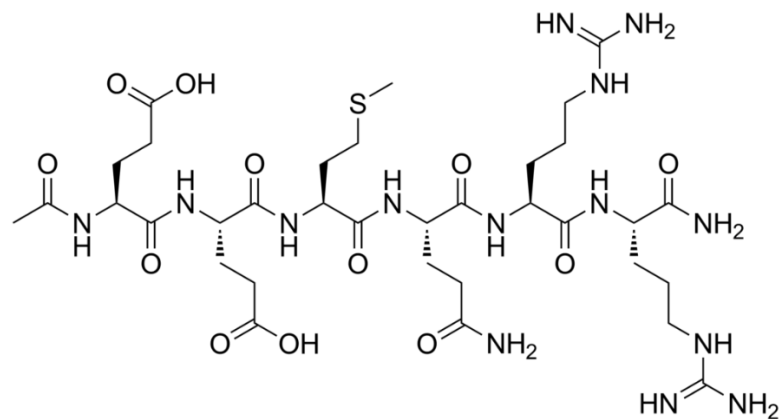
Ac-Glu-Glu-Met-Gln-Arg-Arg-NH 2
