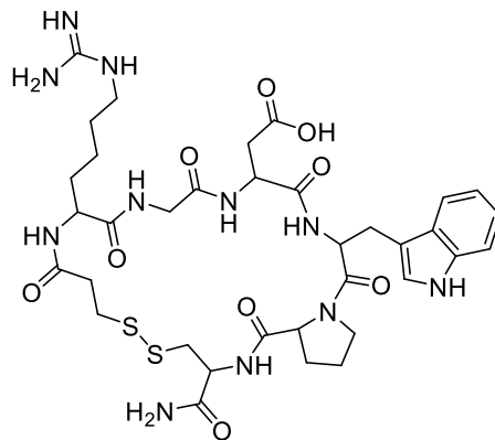
Mpr-Har-Gly-Asp-Trp-Pro-Cys-NH 2
