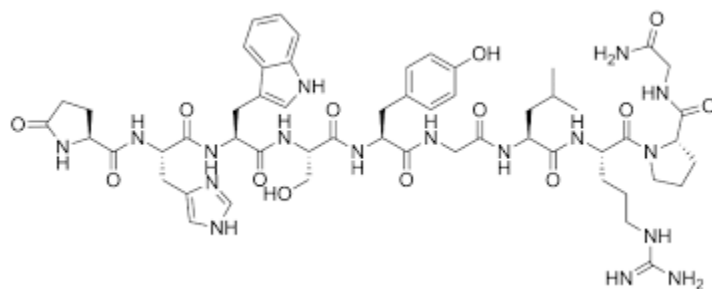
H-Pyr-His-Trp-Ser-Tyr-Gly-Leu-Arg-Pro-Gly-NH 2
