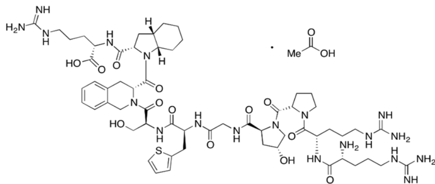
D-Arg-Arg-Pro-Hyp-Gly-Thi-Ser-Tic-Oic-Arg
